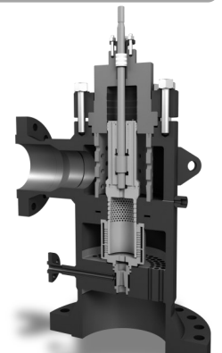
Valve with Drilled Hole Cage & De-Laval Nozzle
