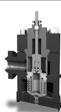
Valve with Zick Twist & De-Laval Nozzle
