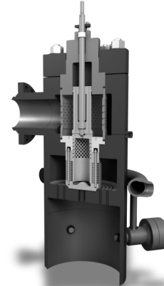
Valve with Zick Twist Cage
