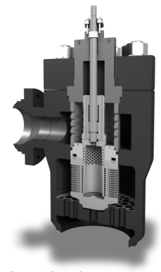
Valve with Zick Twist Cage and SL Nozzle
